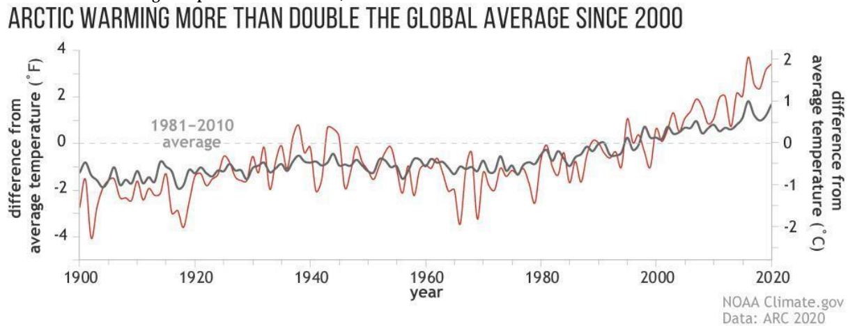
Figure 1. Difference from average temperature in the Arctic, 1900-2020.
